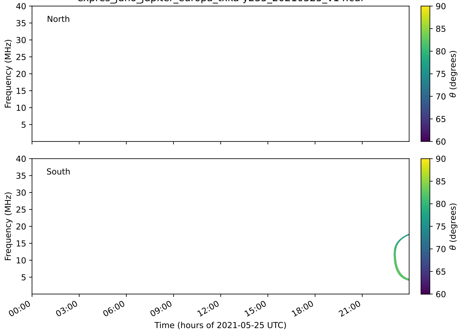
expres_juno_jupiter_europa_txka-y235_20210525_v14.cdf
