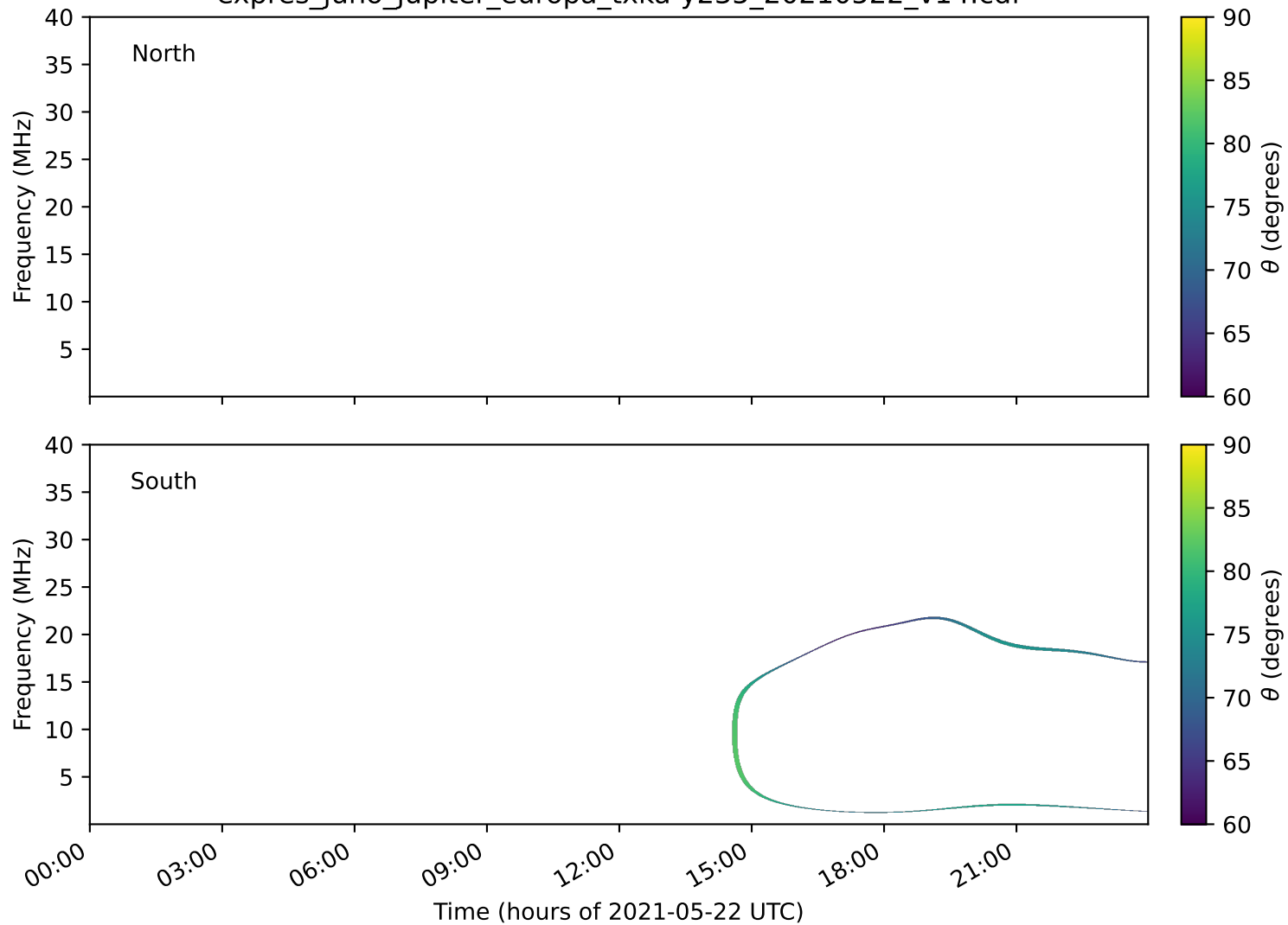
expres_juno_jupiter_europa_txka-y235_20210522_v14.cdf
