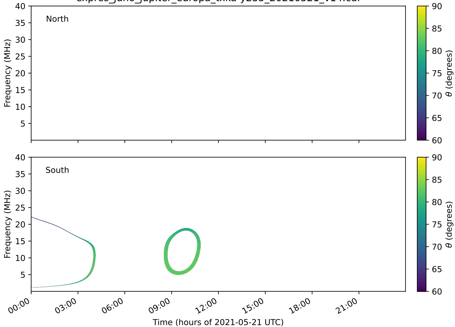
expres_juno_jupiter_europa_txka-y235_20210521_v14.cdf
