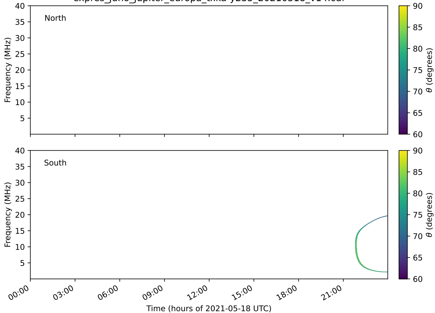
expres_juno_jupiter_europa_txka-y235_20210518_v14.cdf
