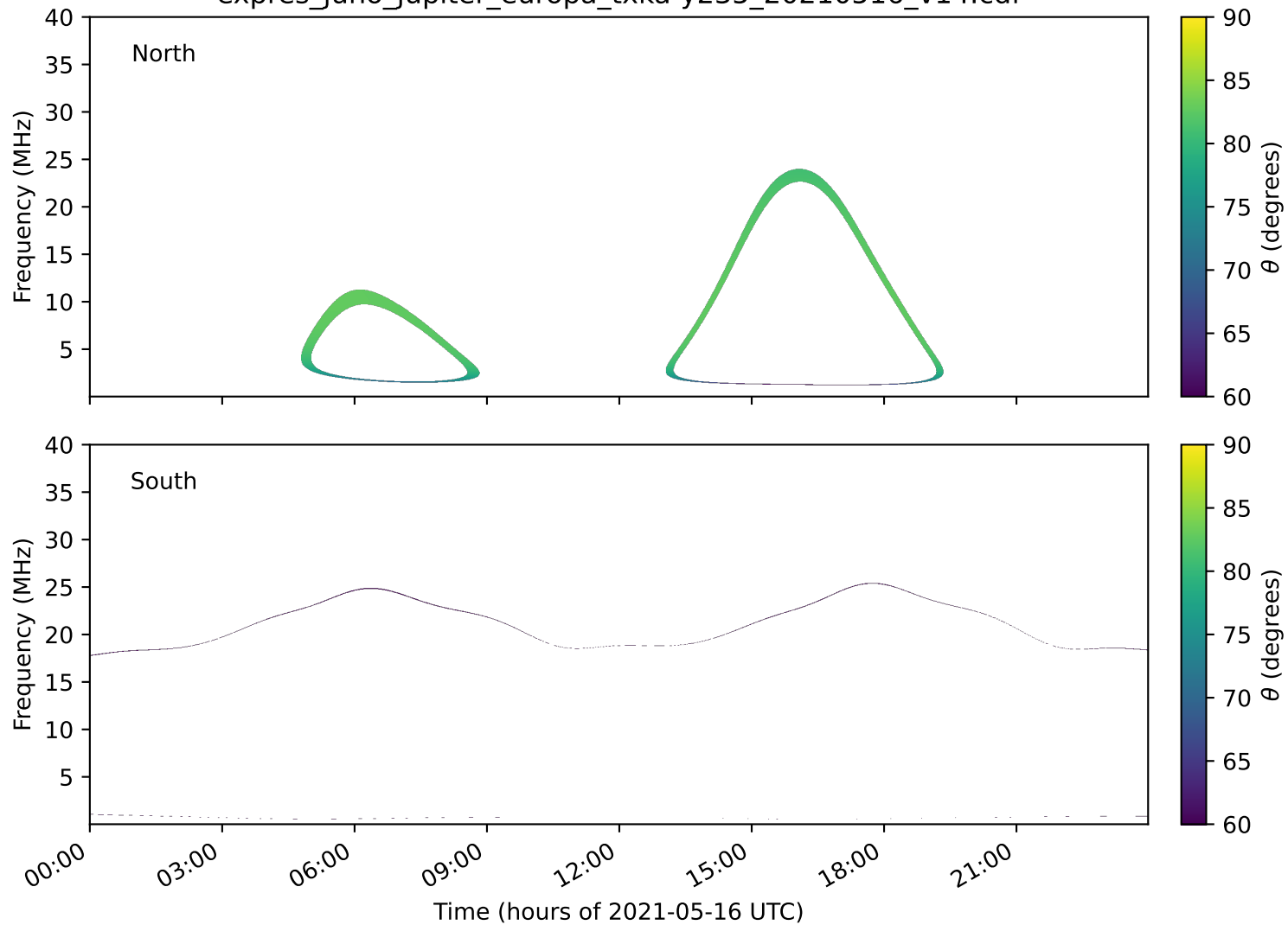
expres_juno_jupiter_europa_txka-y235_20210516_v14.cdf
