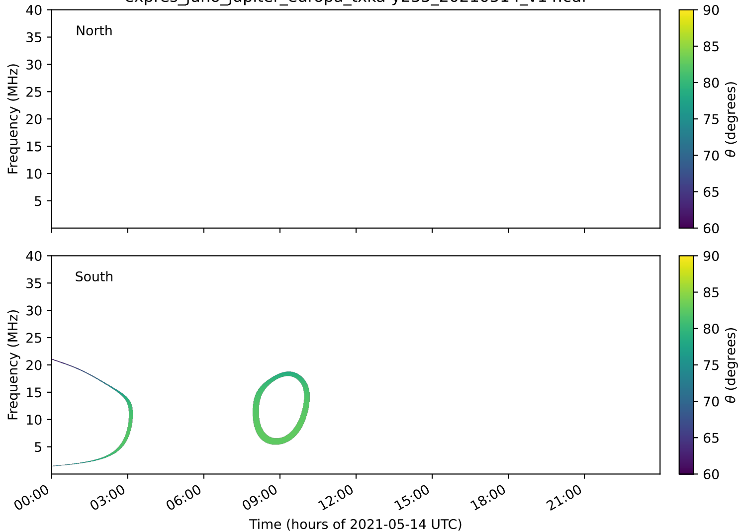
expres_juno_jupiter_europa_txka-y235_20210514_v14.cdf
