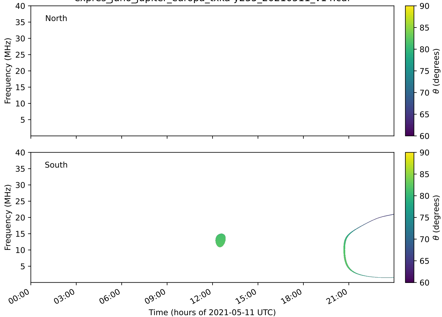
expres_juno_jupiter_europa_txka-y235_20210511_v14.cdf
