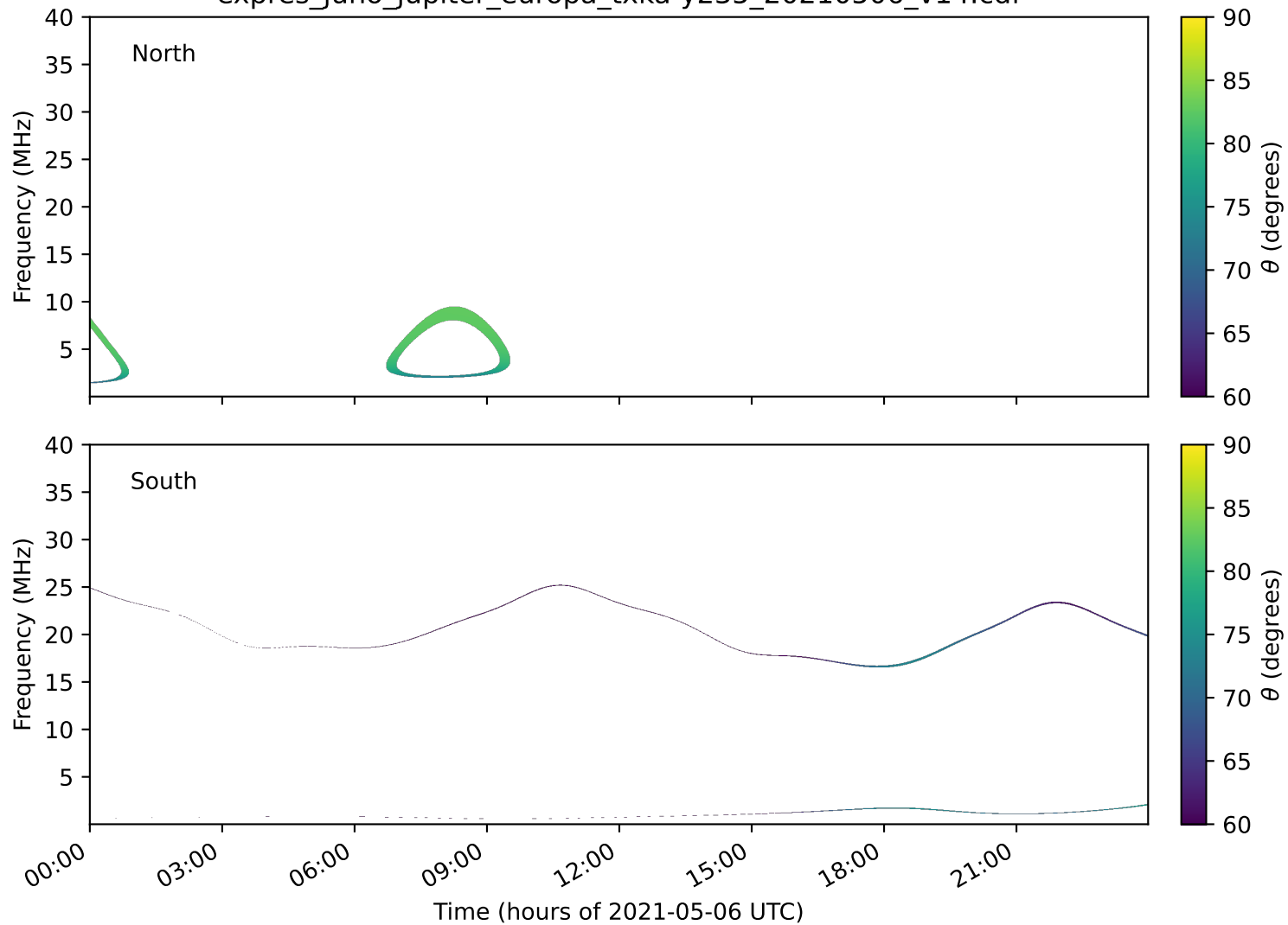
expres_juno_jupiter_europa_txka-y235_20210506_v14.cdf
