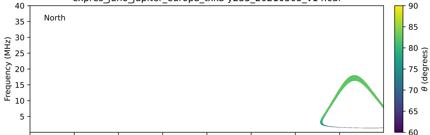
expres_juno_jupiter_europa_txka-y235_20210505_v14.cdf
