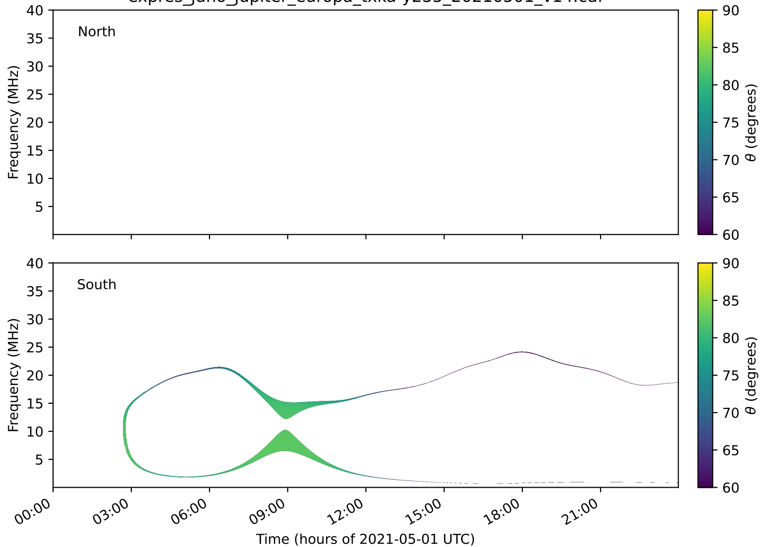
expres_juno_jupiter_europa_txka-y235_20210501_v14.cdf
