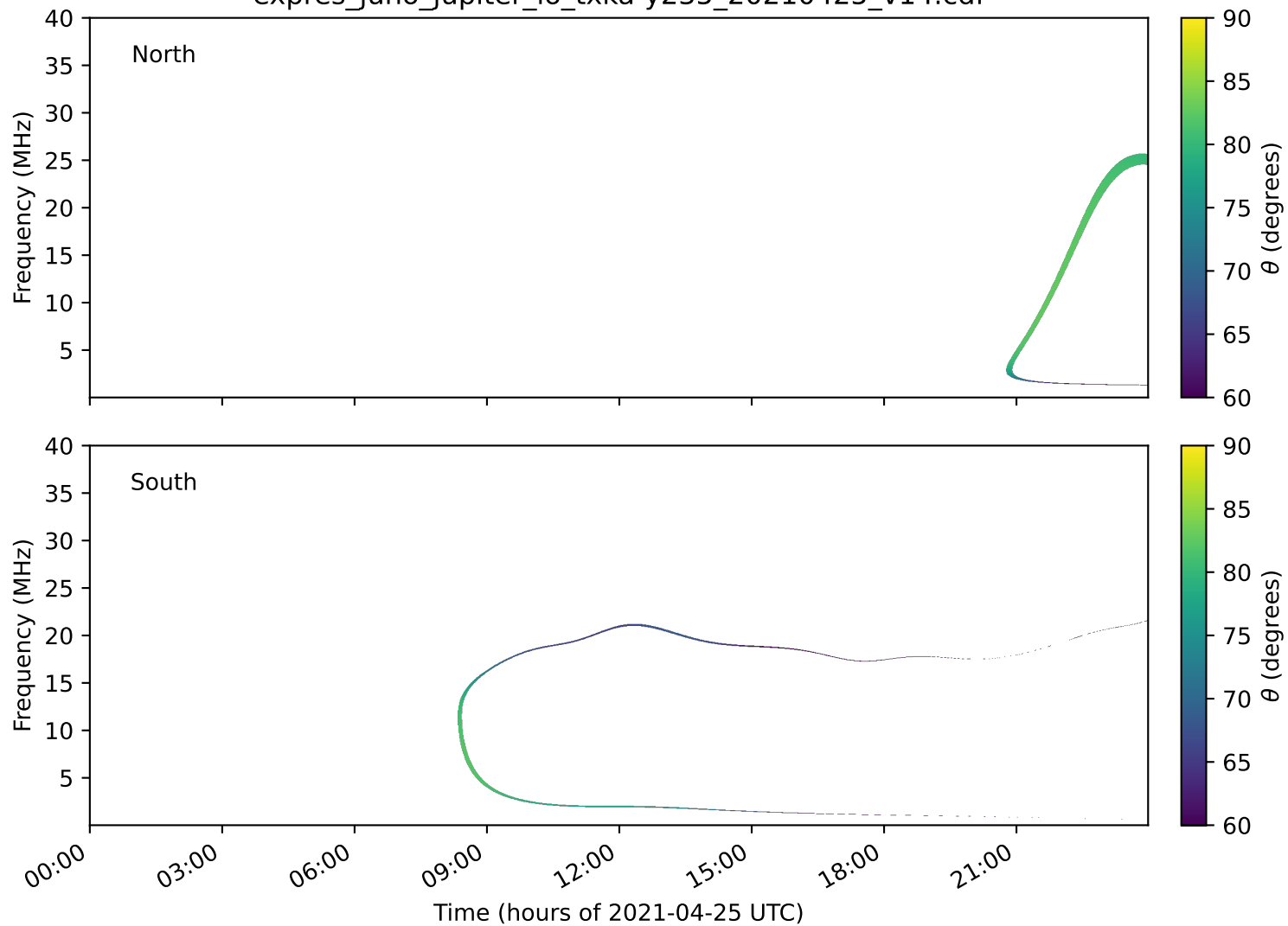
expres_juno_jupiter_io_txka-y235_20210425_v14.cdf
