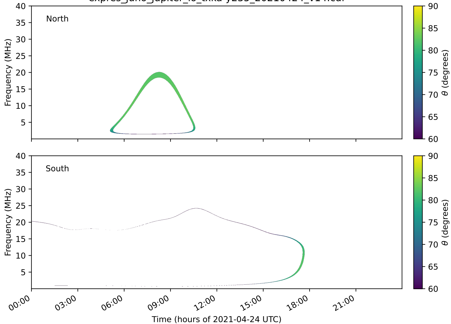
expres_juno_jupiter_io_txka-y235_20210424_v14.cdf
