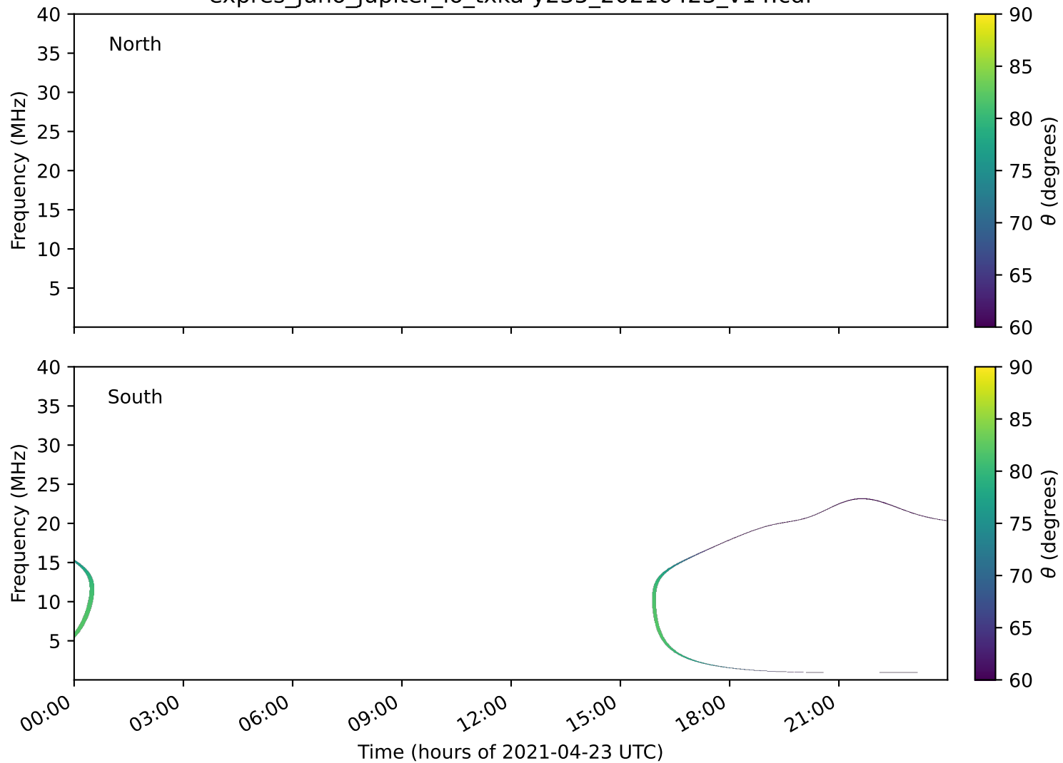
expres_juno_jupiter_io_txka-y235_20210423_v14.cdf
