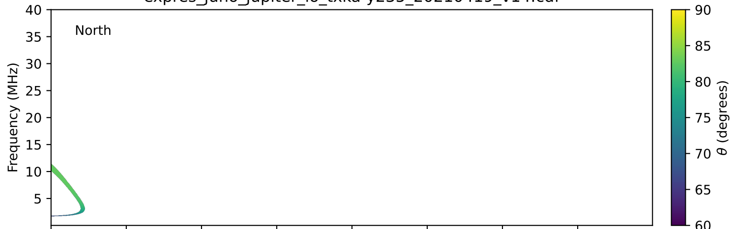
expres_juno_jupiter_io_txka-y235_20210419_v14.cdf
