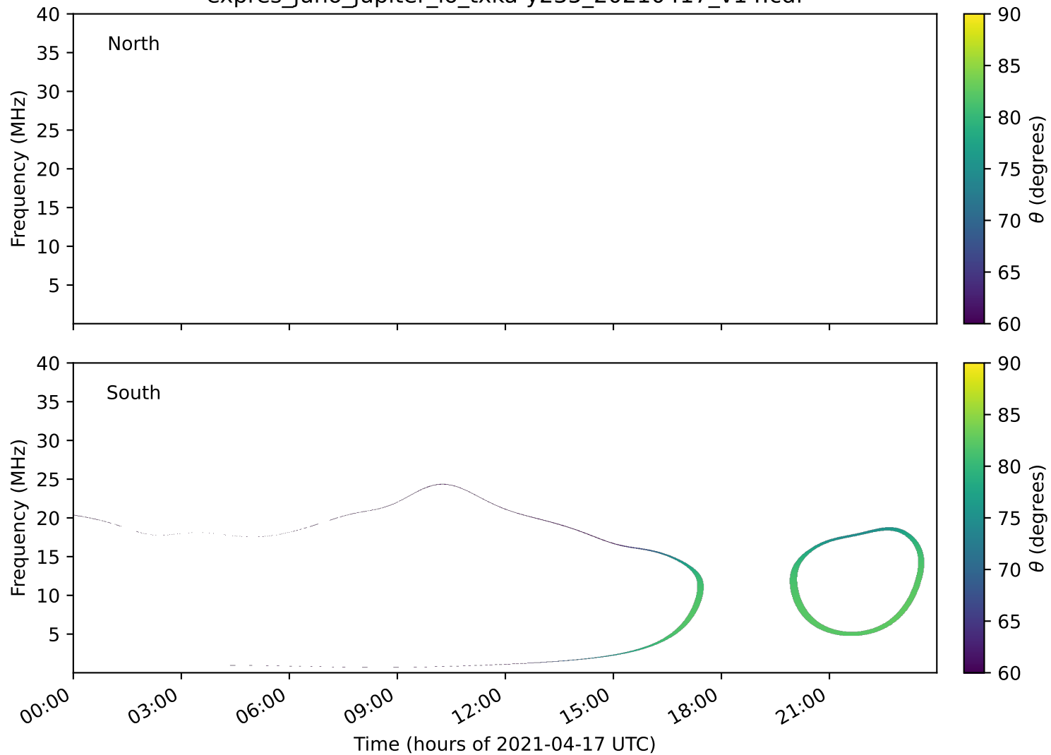
expres_juno_jupiter_io_txka-y235_20210417_v14.cdf
