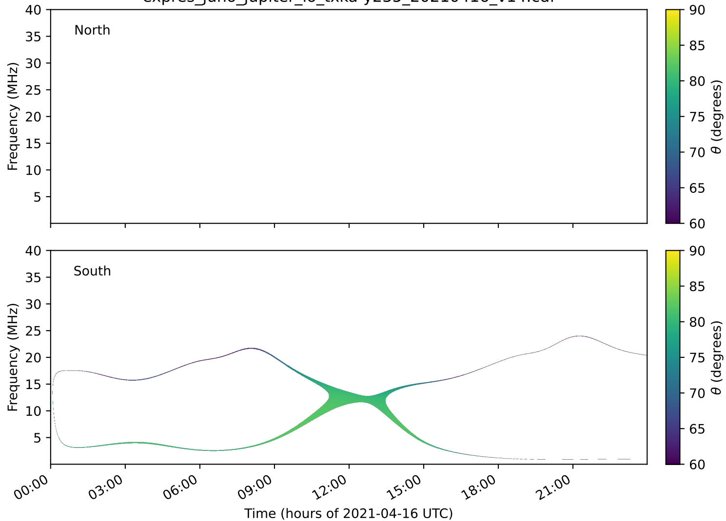
expres_juno_jupiter_io_txka-y235_20210416_v14.cdf
