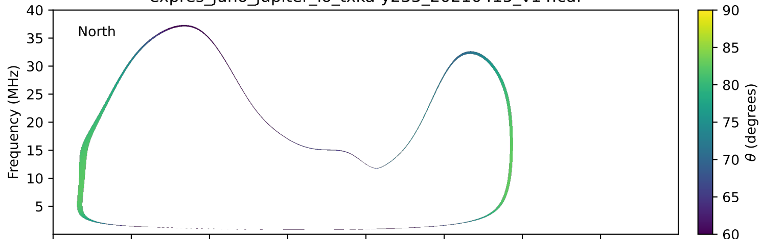
expres_juno_jupiter_io_txka-y235_20210415_v14.cdf
