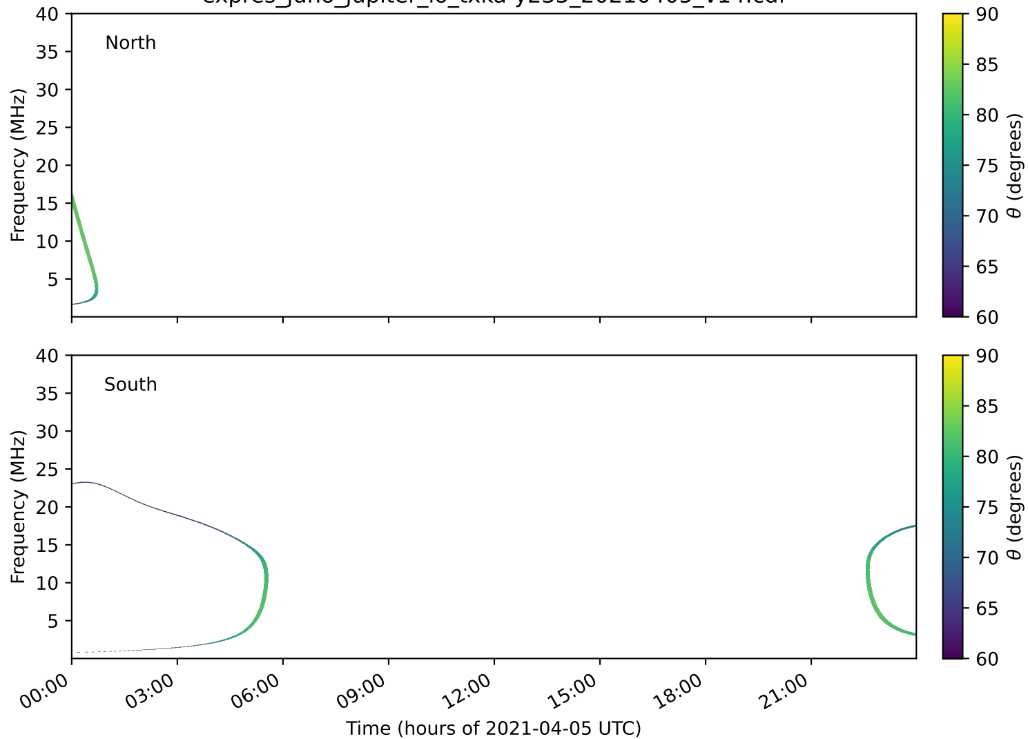
expres_juno_jupiter_io_txka-y235_20210405_v14.cdf
