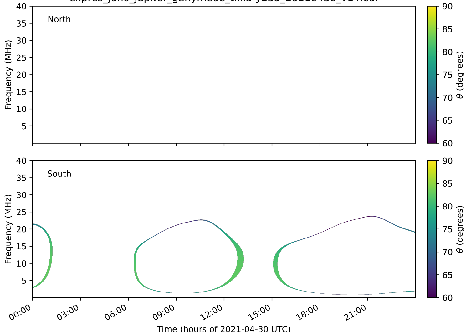
expres_juno_jupiter_ganymede_txka-y235_20210430_v14.cdf
