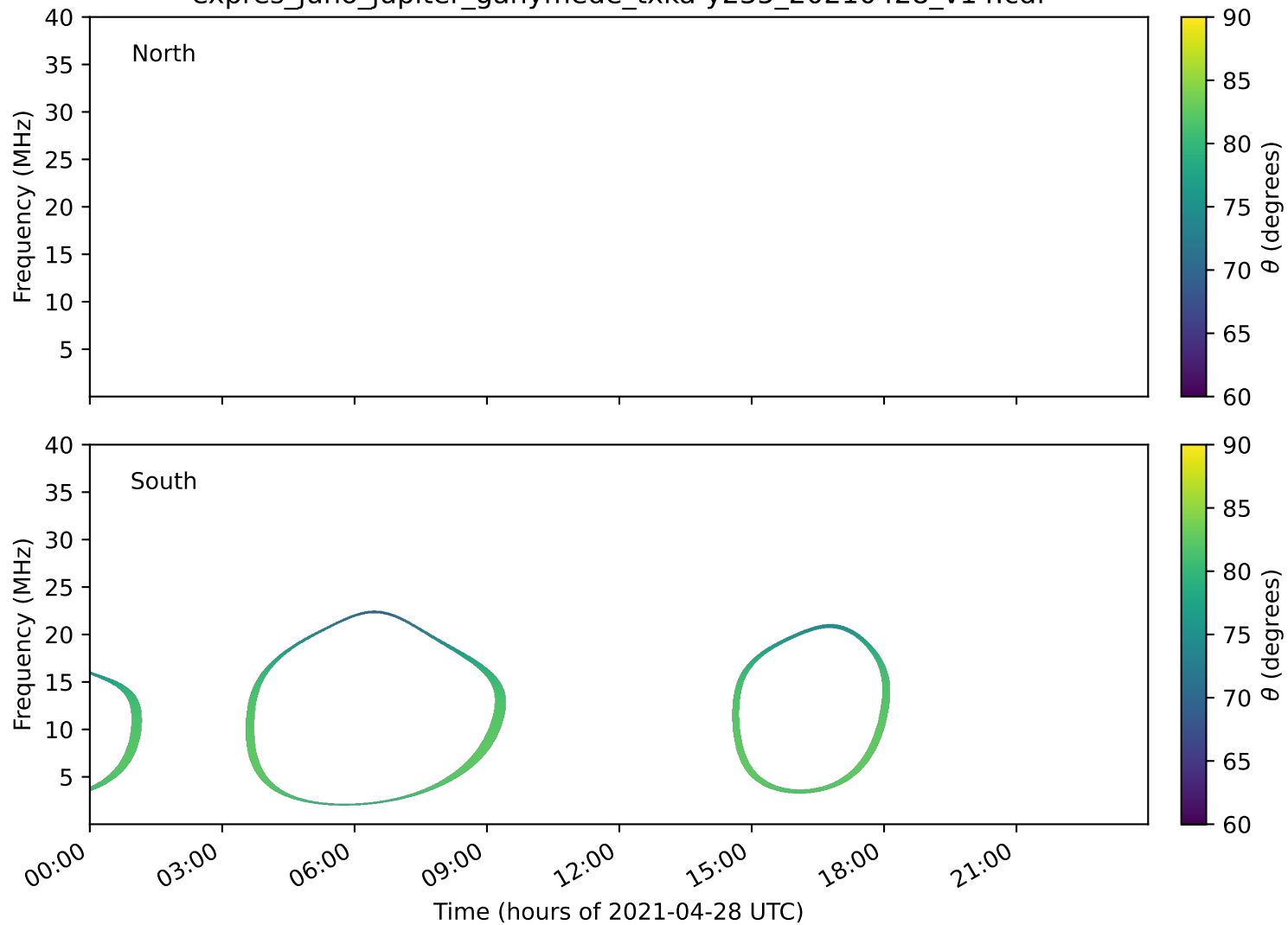
expres_juno_jupiter_ganymede_txka-y235_20210428_v14.cdf
