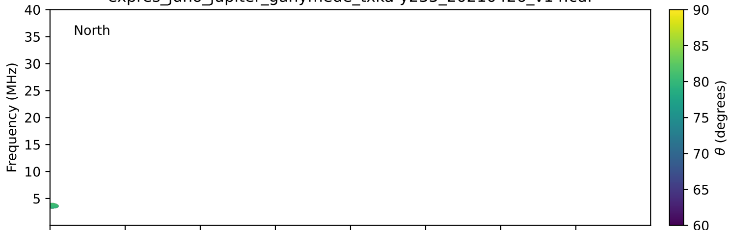
expres_juno_jupiter_ganymede_txka-y235_20210426_v14.cdf
