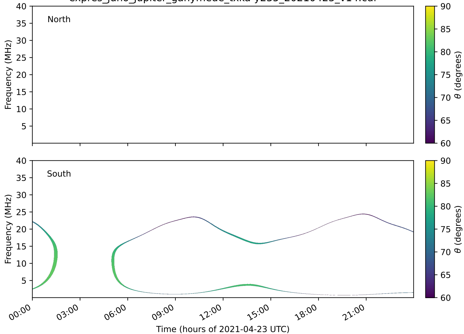
expres_juno_jupiter_ganymede_txka-y235_20210423_v14.cdf
