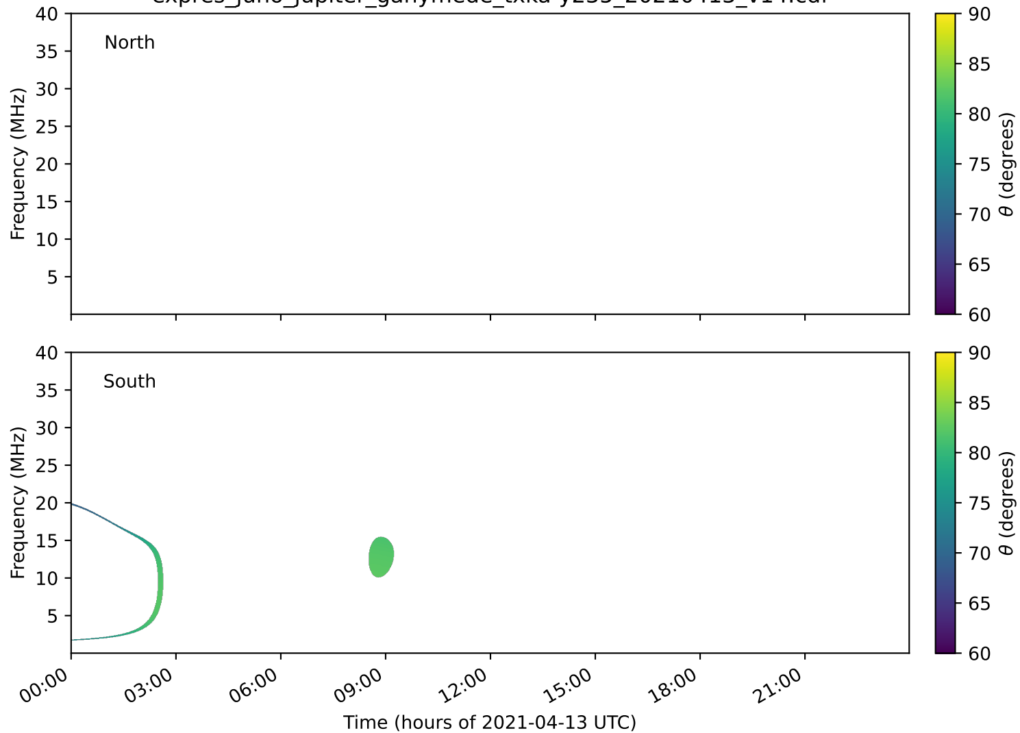
expres_juno_jupiter_ganymede_txka-y235_20210413_v14.cdf
