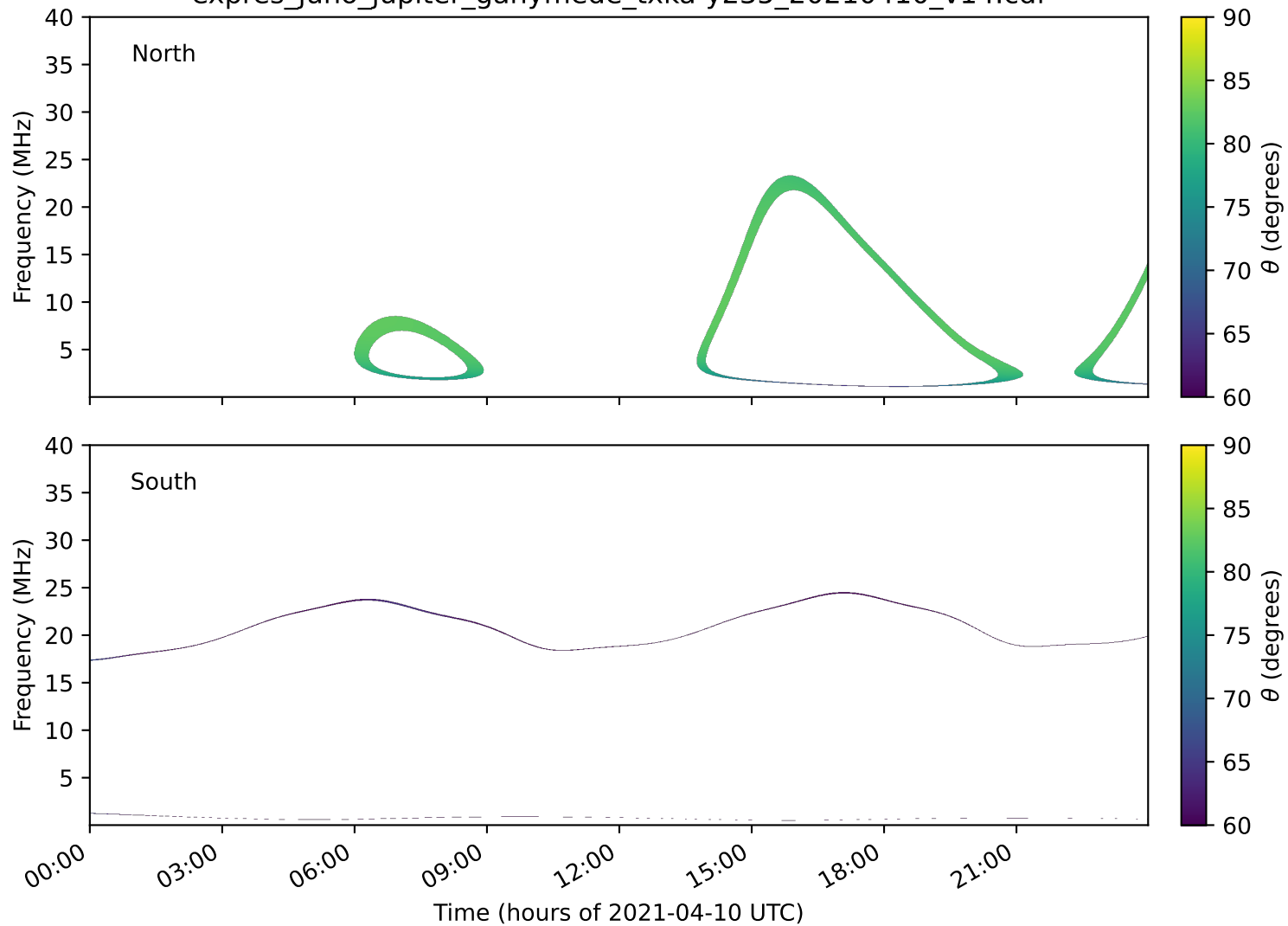
expres_juno_jupiter_ganymede_txka-y235_20210410_v14.cdf
