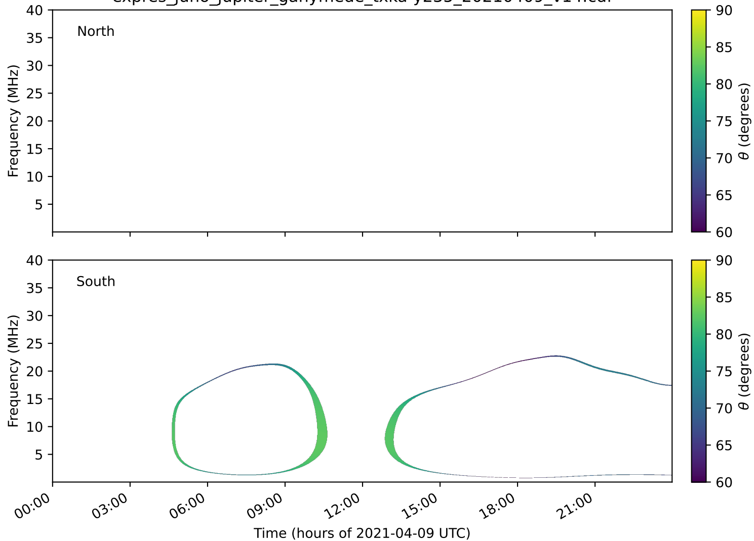
expres_juno_jupiter_ganymede_txka-y235_20210409_v14.cdf
