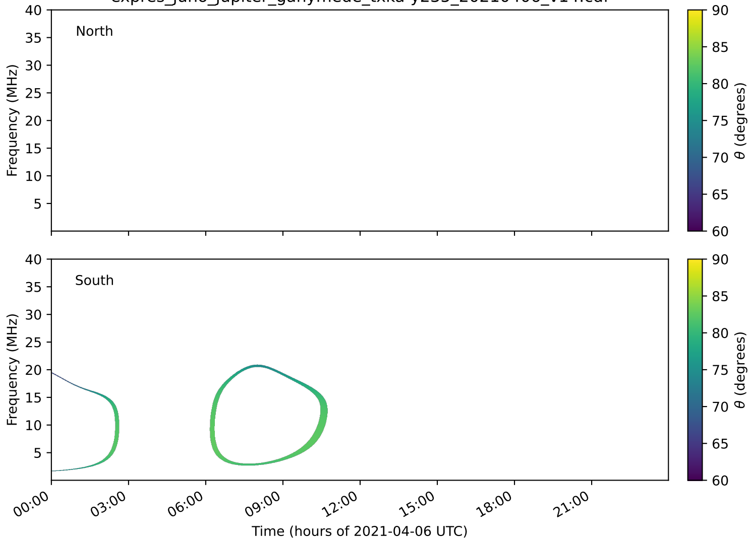
expres_juno_jupiter_ganymede_txka-y235_20210406_v14.cdf
