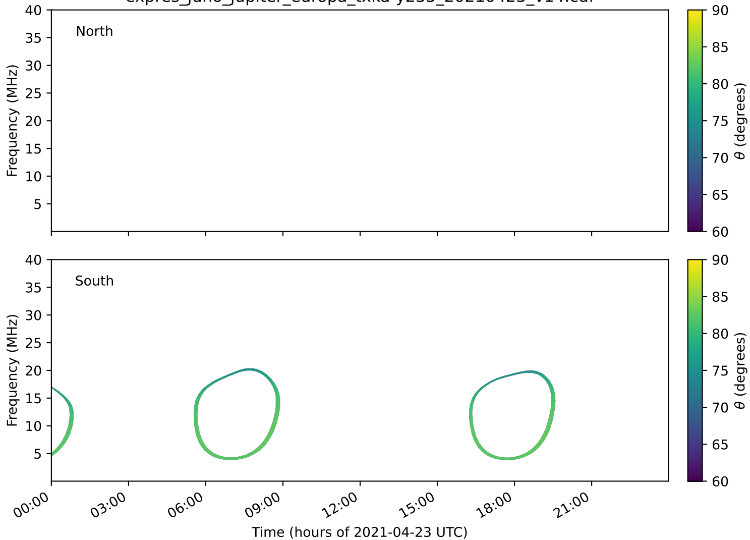
expres_juno_jupiter_europa_txka-y235_20210423_v14.cdf
