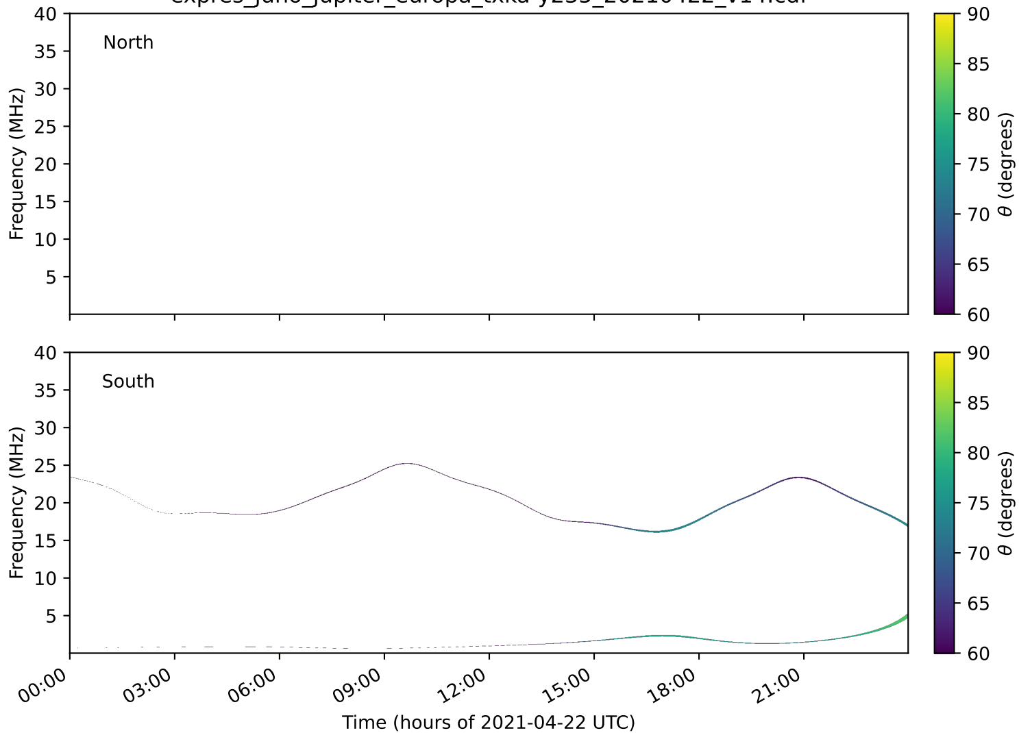
expres_juno_jupiter_europa_txka-y235_20210422_v14.cdf
