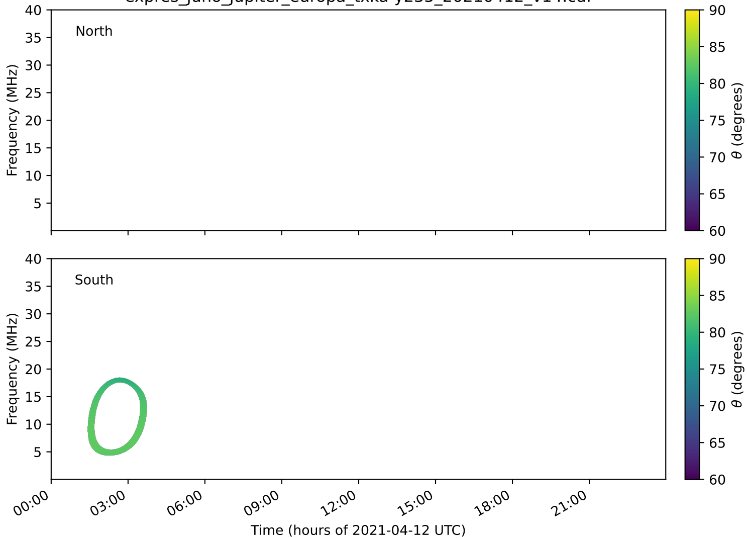
expres_juno_jupiter_europa_txka-y235_20210412_v14.cdf
