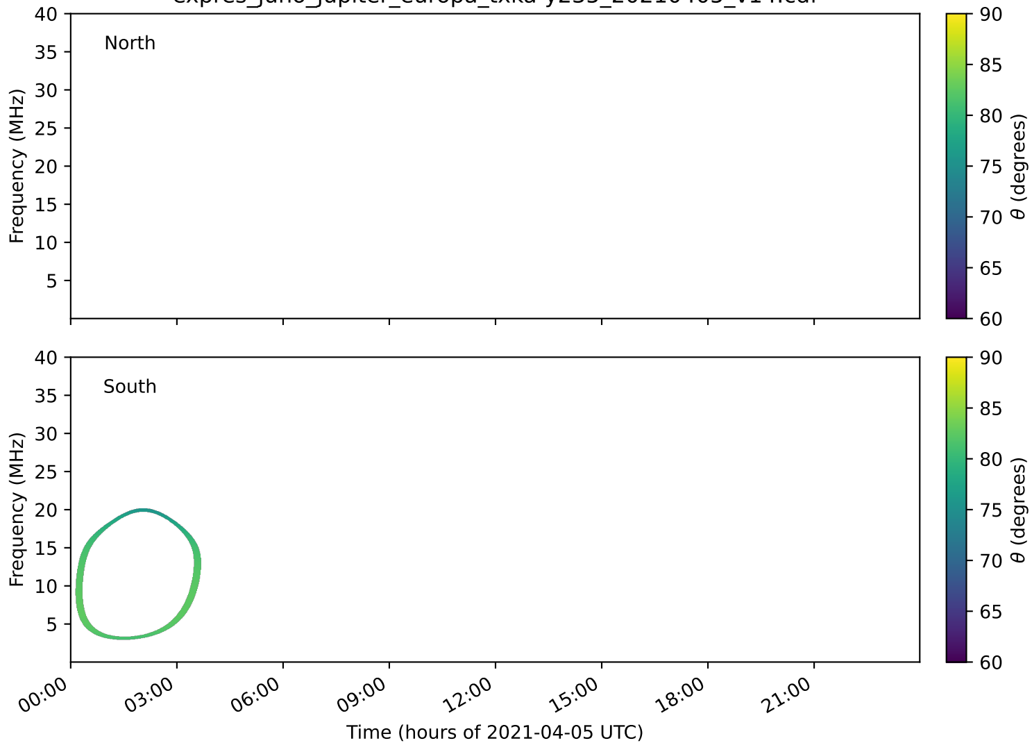
expres_juno_jupiter_europa_txka-y235_20210405_v14.cdf
