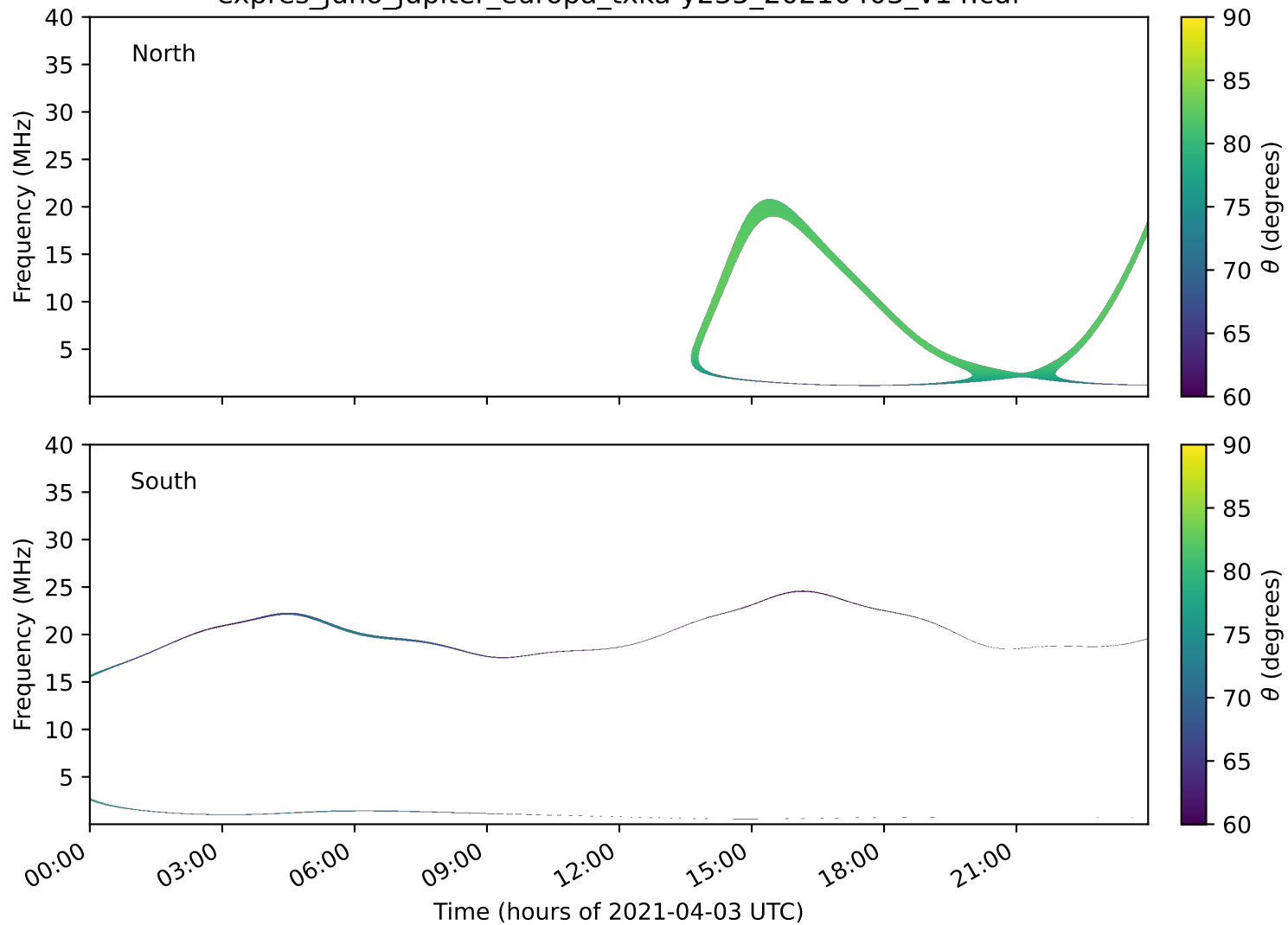
expres_juno_jupiter_europa_txka-y235_20210403_v14.cdf
