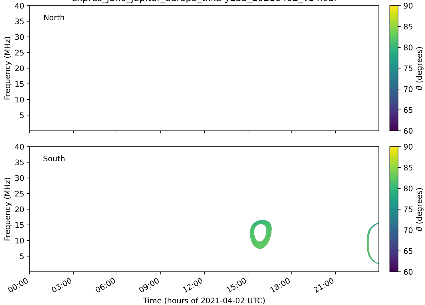
expres_juno_jupiter_europa_txka-y235_20210402_v14.cdf
