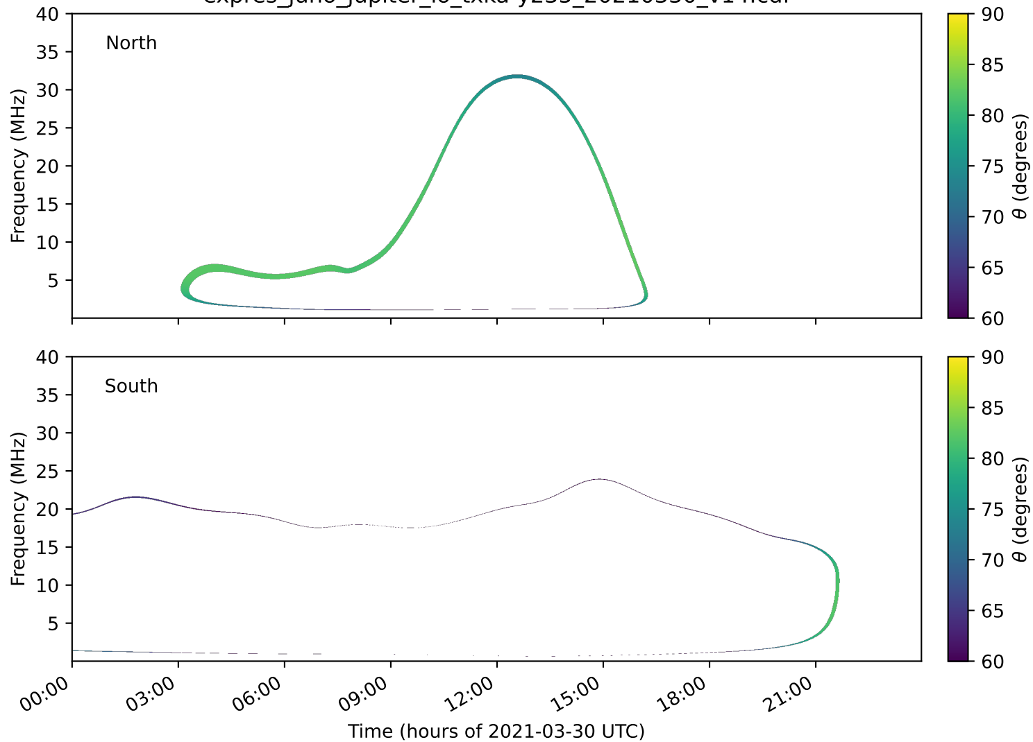
expres_juno_jupiter_io_txka-y235_20210330_v14.cdf
