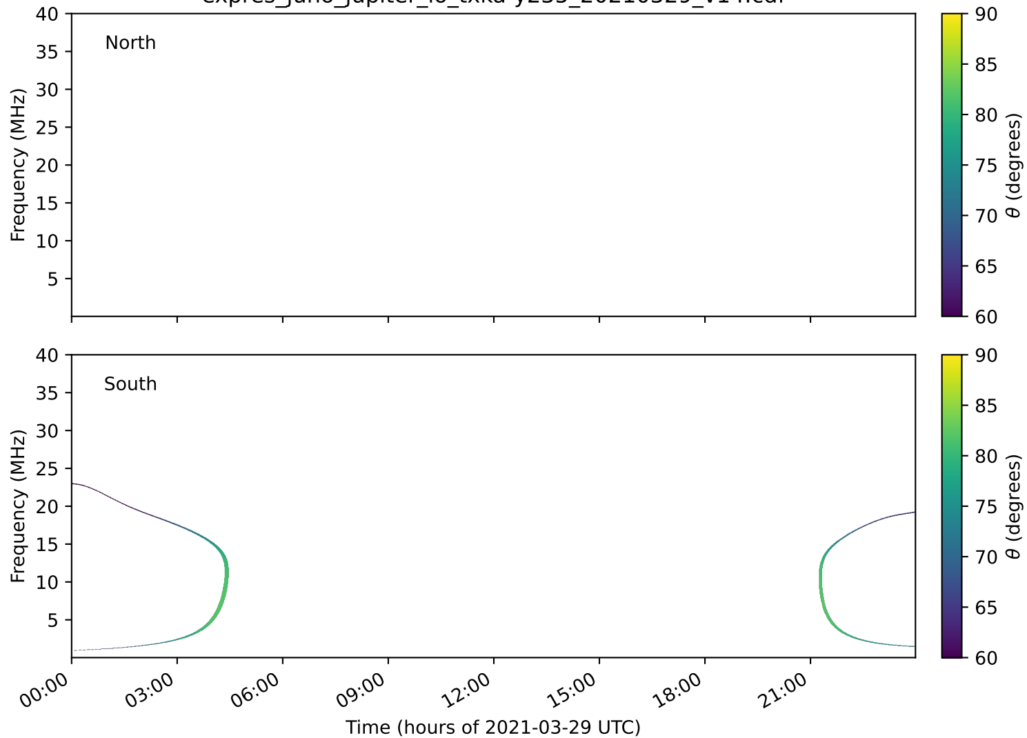
expres_juno_jupiter_io_txka-y235_20210329_v14.cdf
