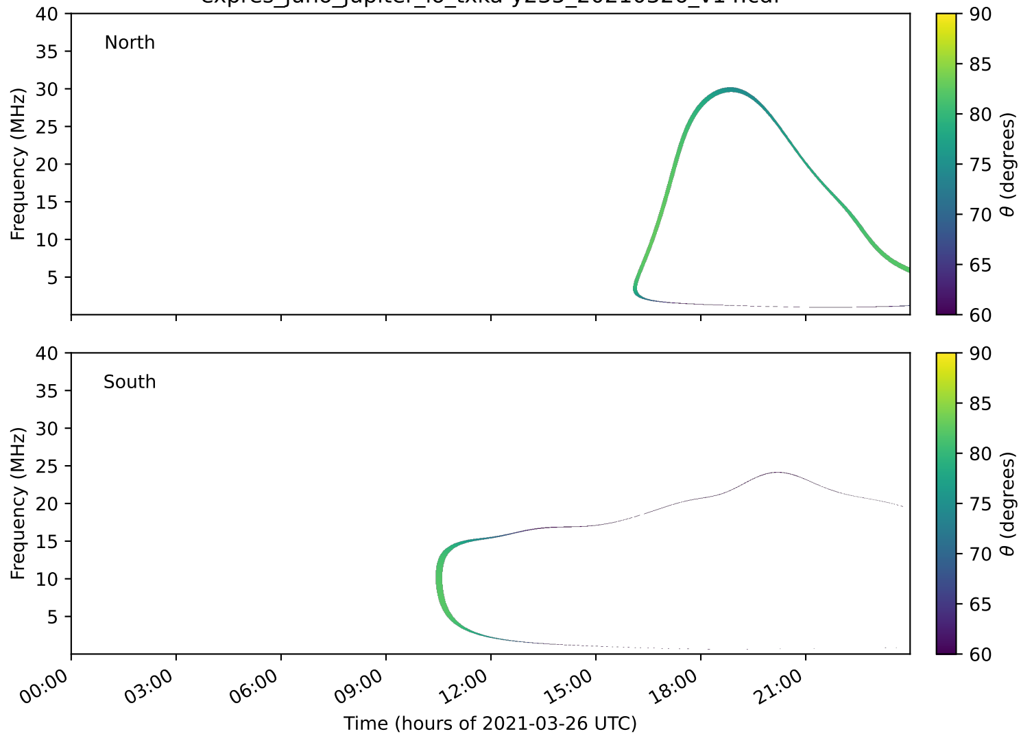
expres_juno_jupiter_io_txka-y235_20210326_v14.cdf
