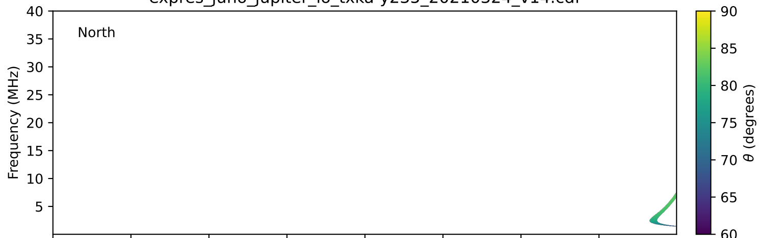
expres_juno_jupiter_io_txka-y235_20210324_v14.cdf
