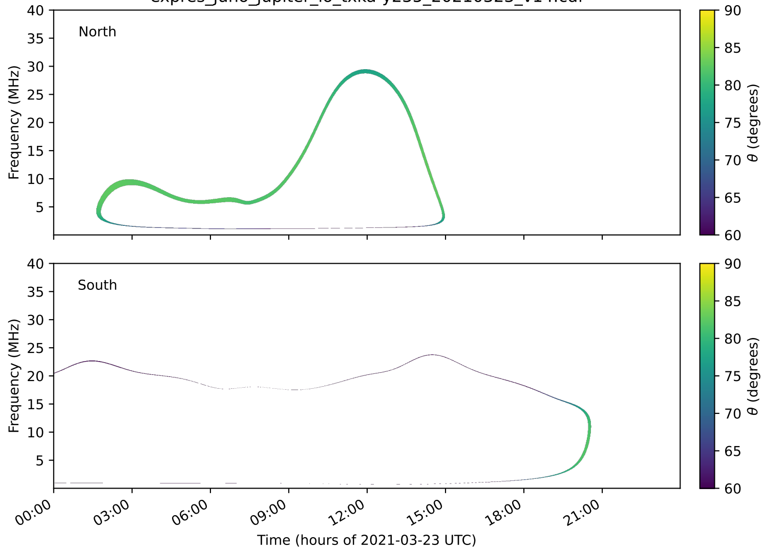
expres_juno_jupiter_io_txka-y235_20210323_v14.cdf
