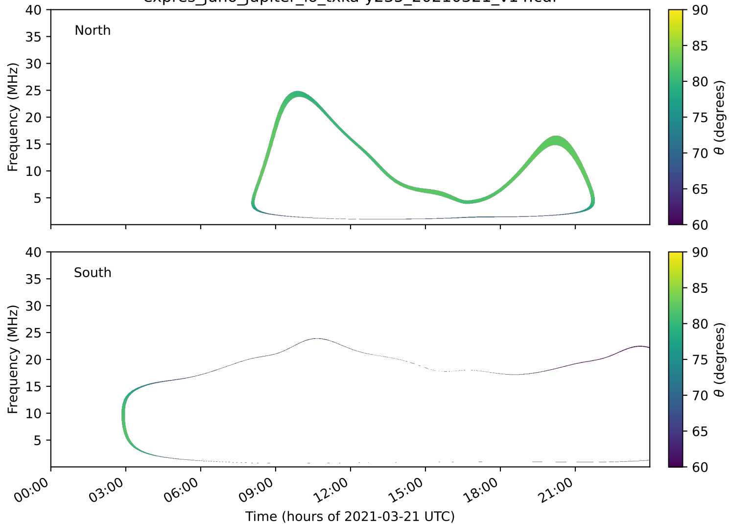
expres_juno_jupiter_io_txka-y235_20210321_v14.cdf
