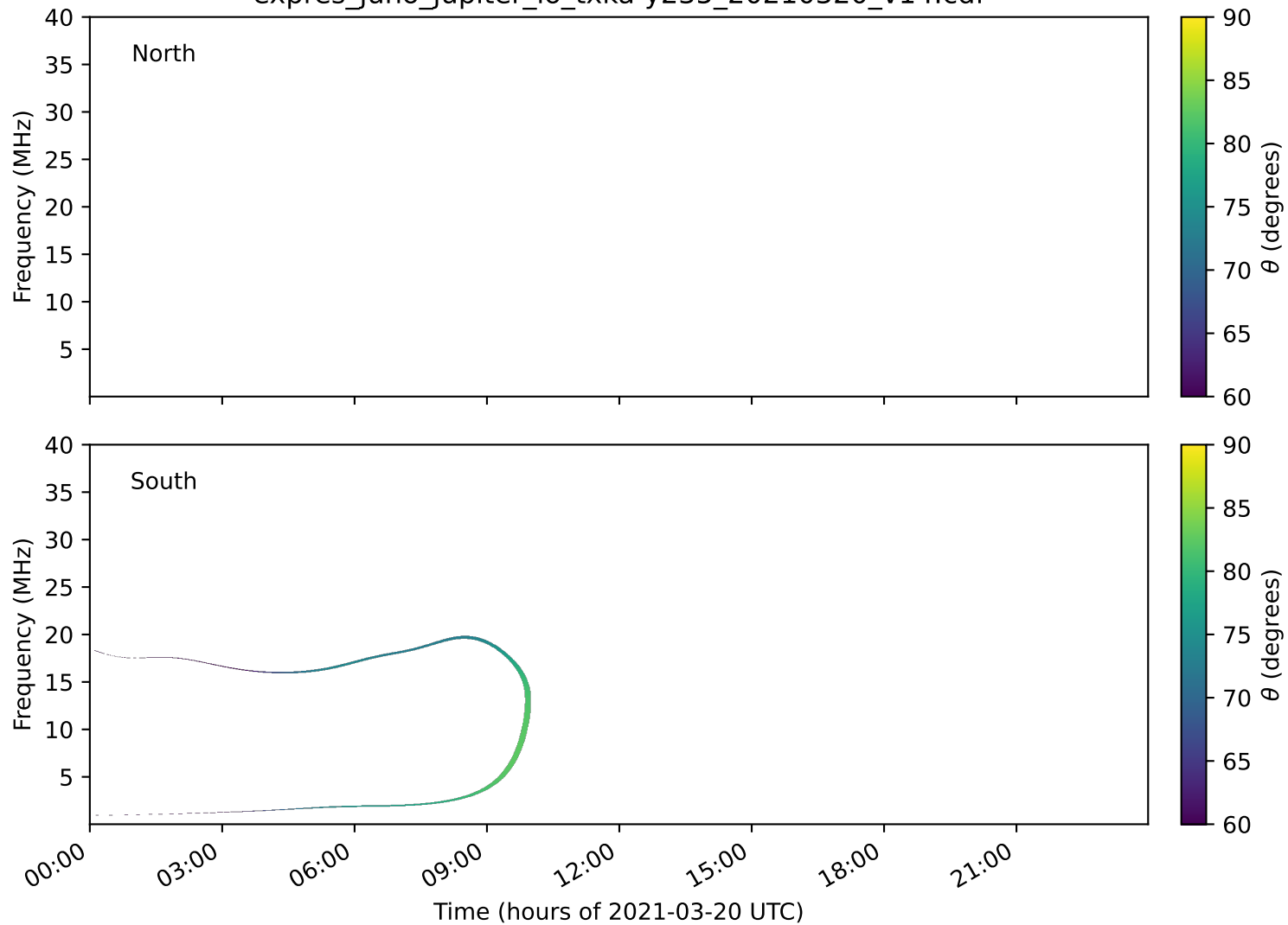
expres_juno_jupiter_io_txka-y235_20210320_v14.cdf
