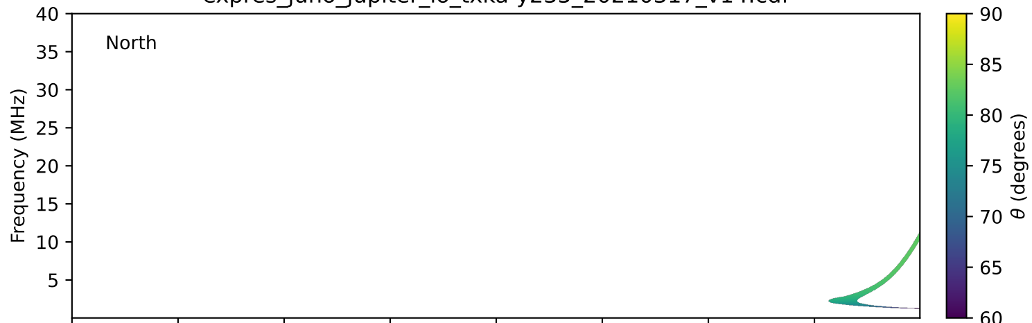
expres_juno_jupiter_io_txka-y235_20210317_v14.cdf
