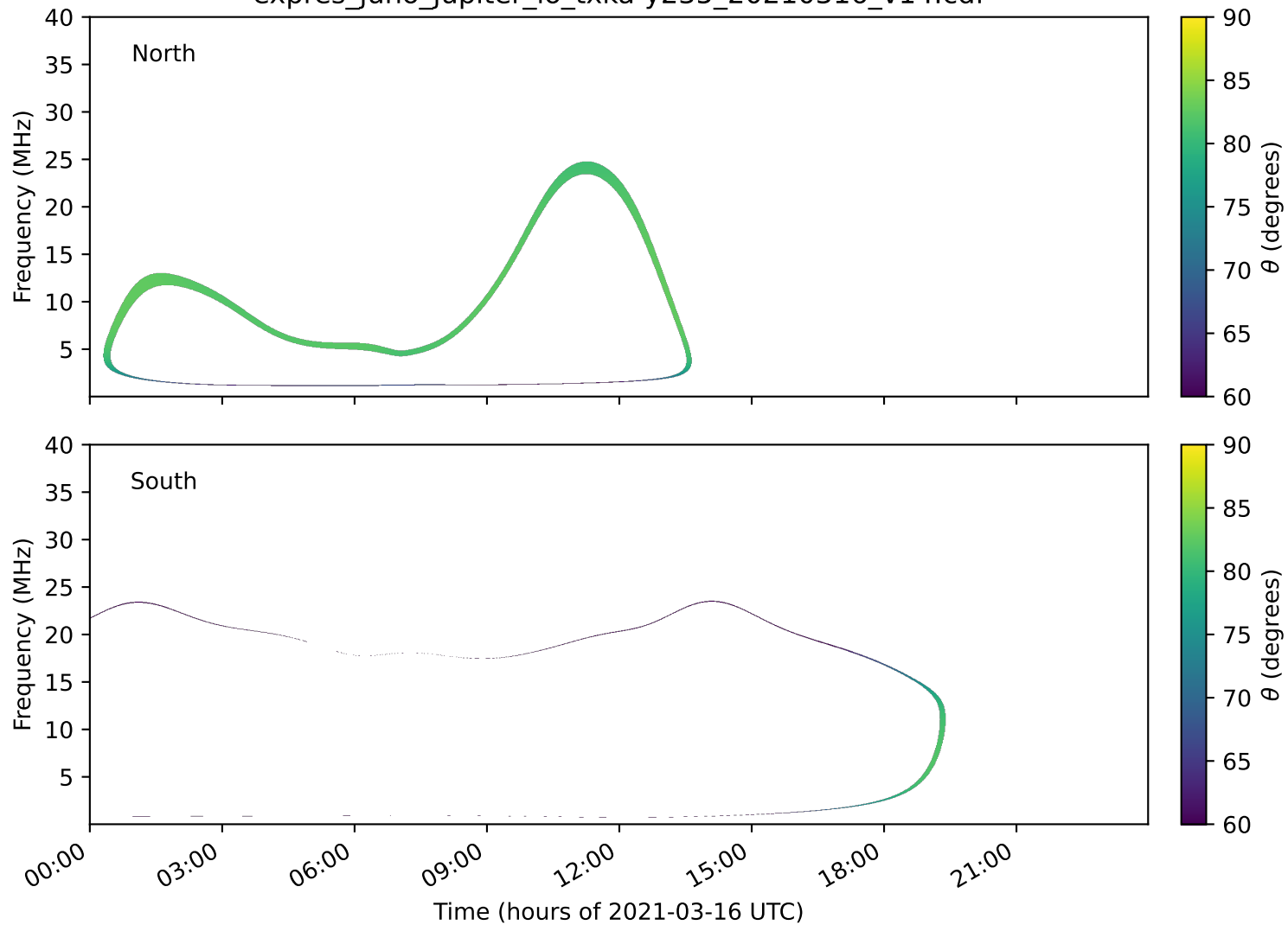
expres_juno_jupiter_io_txka-y235_20210316_v14.cdf
