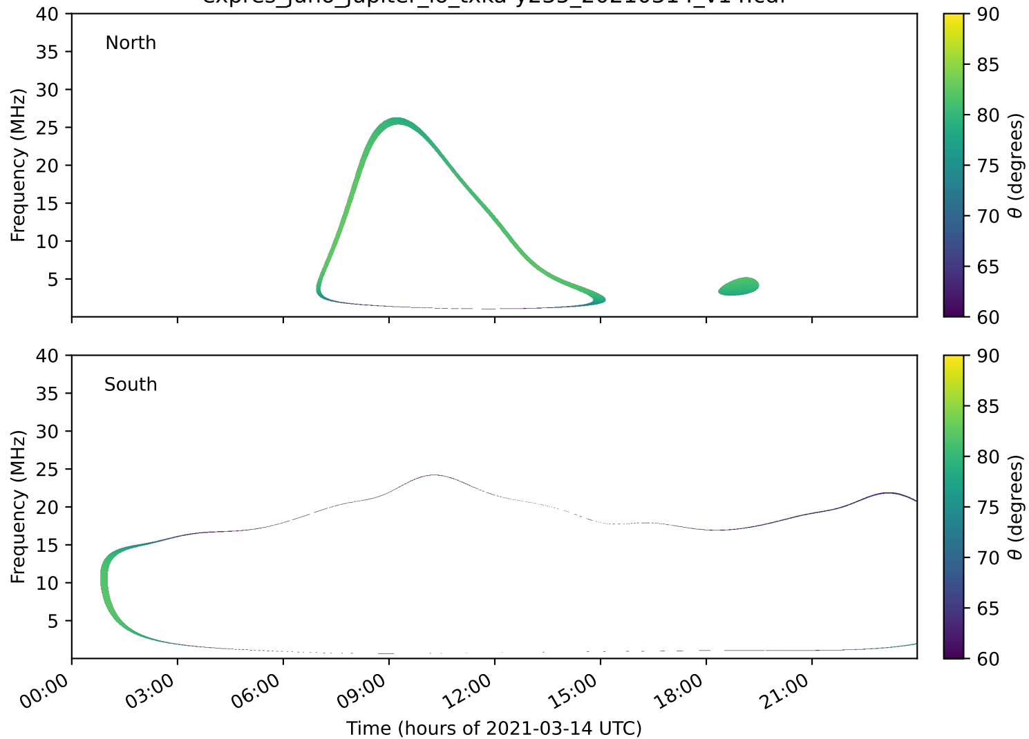
expres_juno_jupiter_io_txka-y235_20210314_v14.cdf
