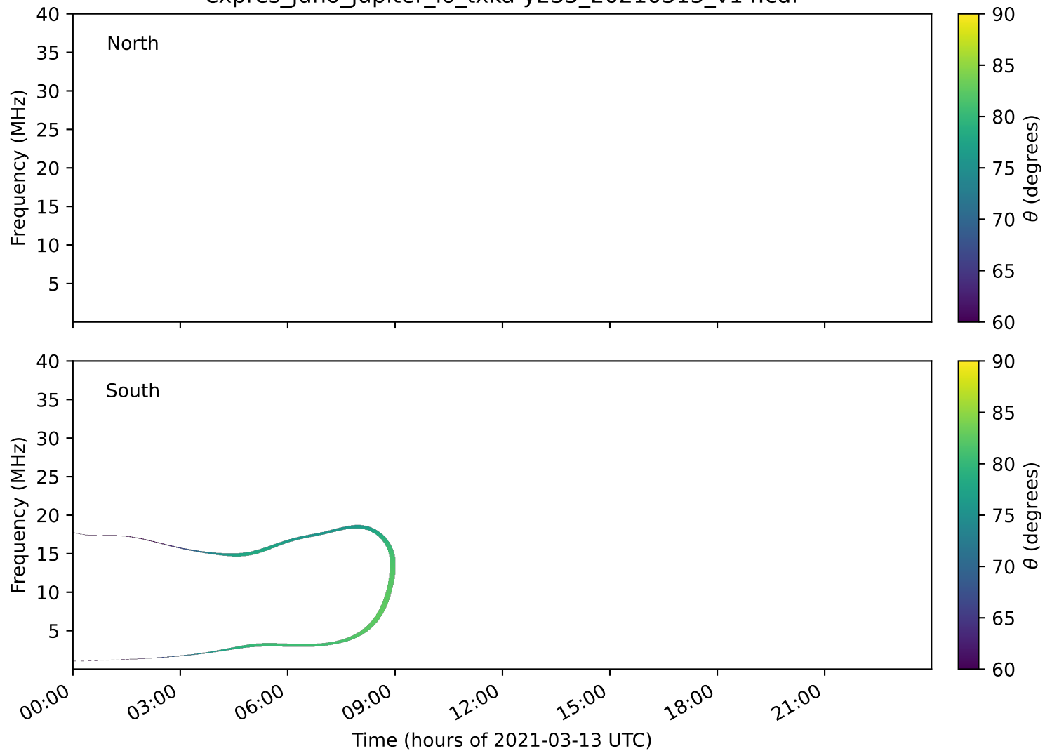
expres_juno_jupiter_io_txka-y235_20210313_v14.cdf
