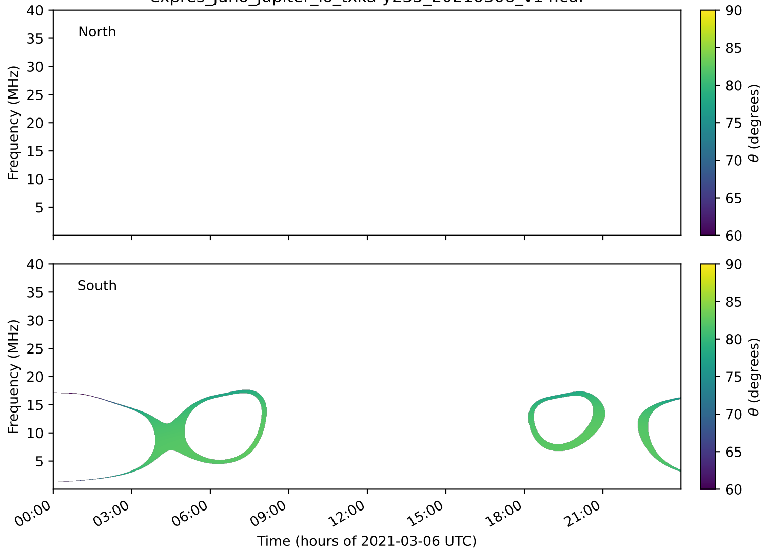
expres_juno_jupiter_io_txka-y235_20210306_v14.cdf
