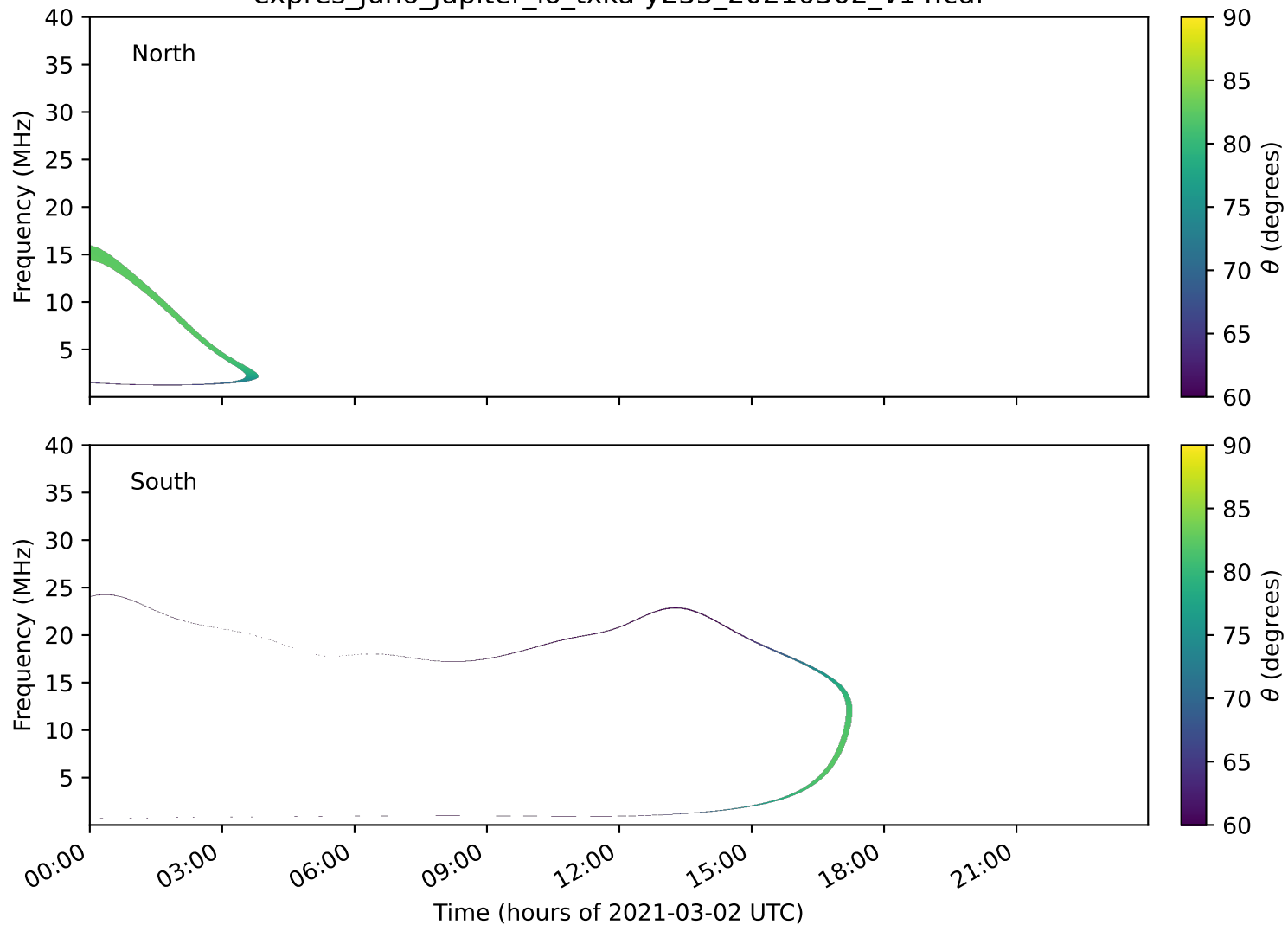
expres_juno_jupiter_io_txka-y235_20210302_v14.cdf
