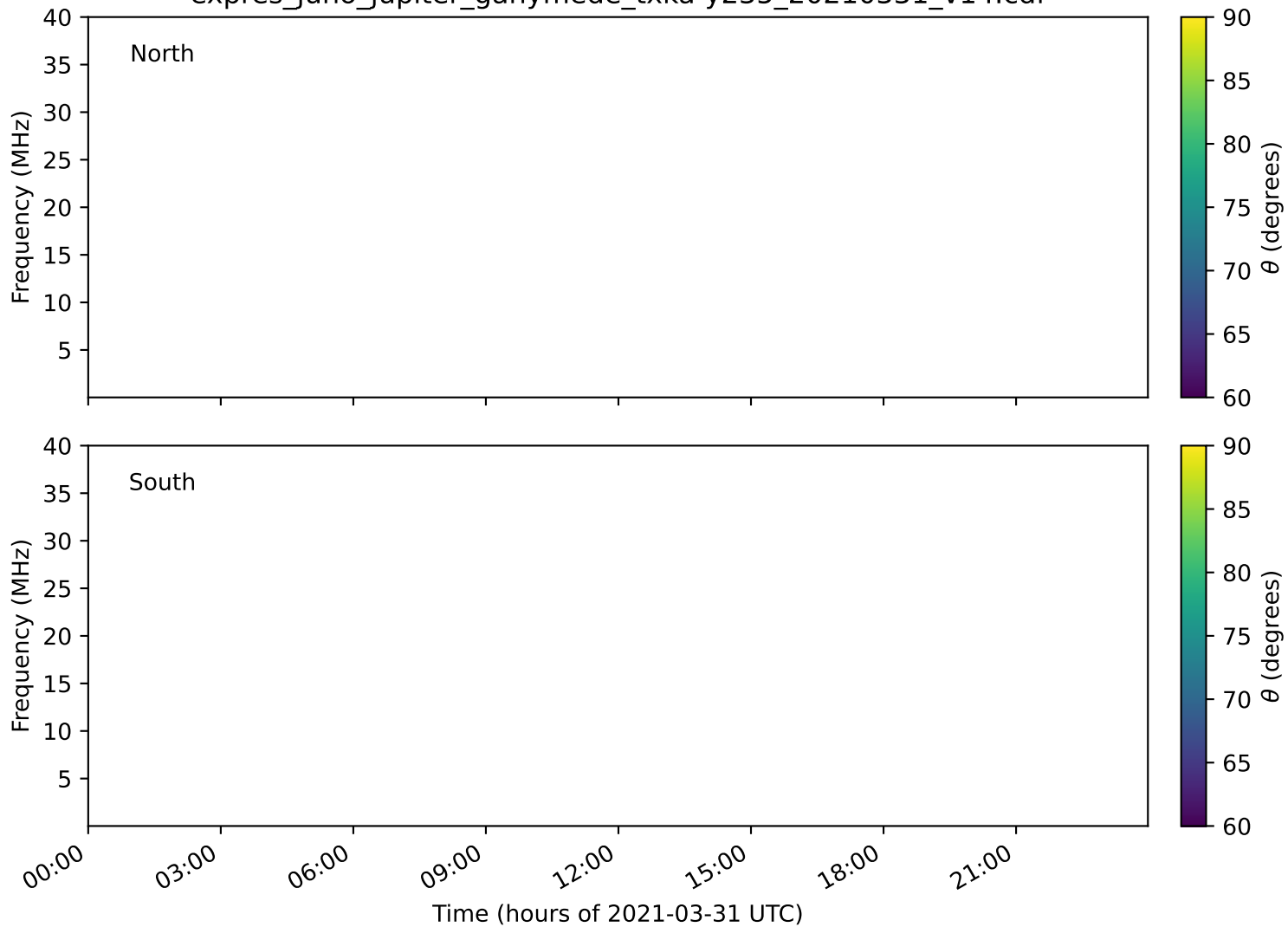
expres_juno_jupiter_ganymede_txka-y235_20210331_v14.cdf
