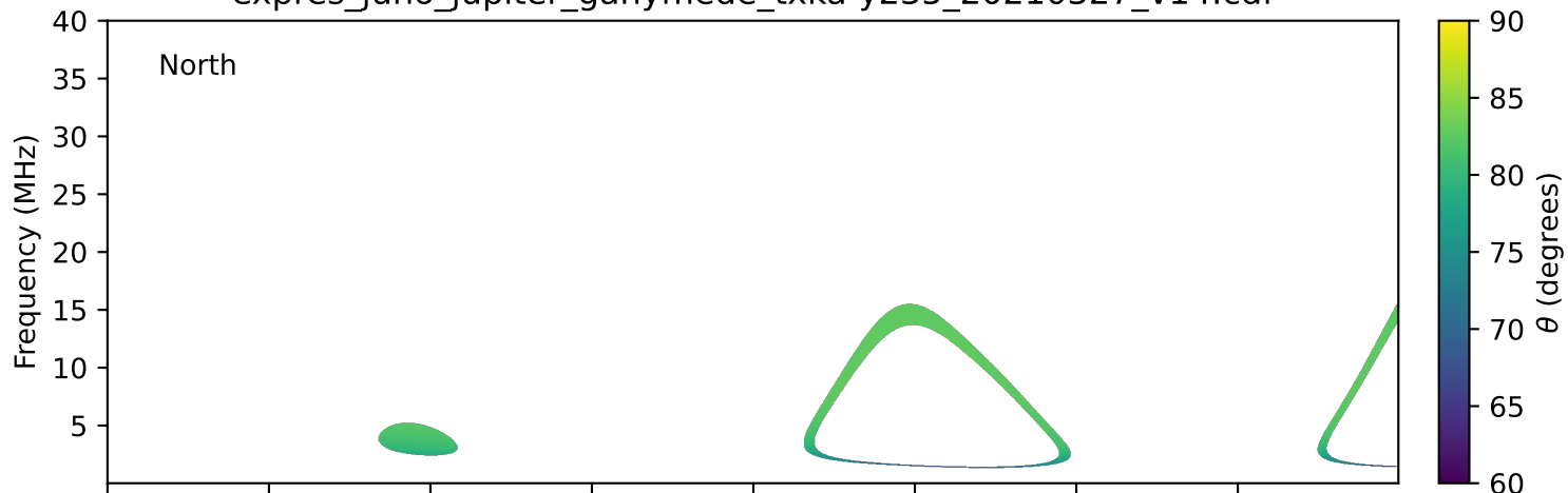
expres_juno_jupiter_ganymede_txka-y235_20210327_v14.cdf
