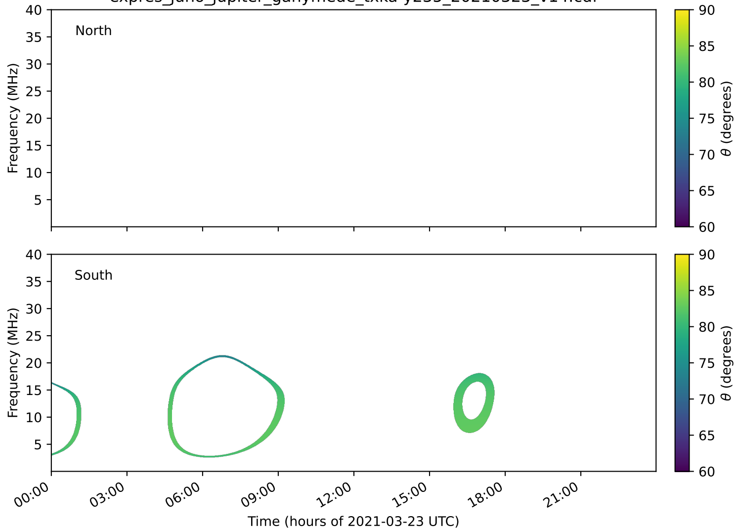
expres_juno_jupiter_ganymede_txka-y235_20210323_v14.cdf
