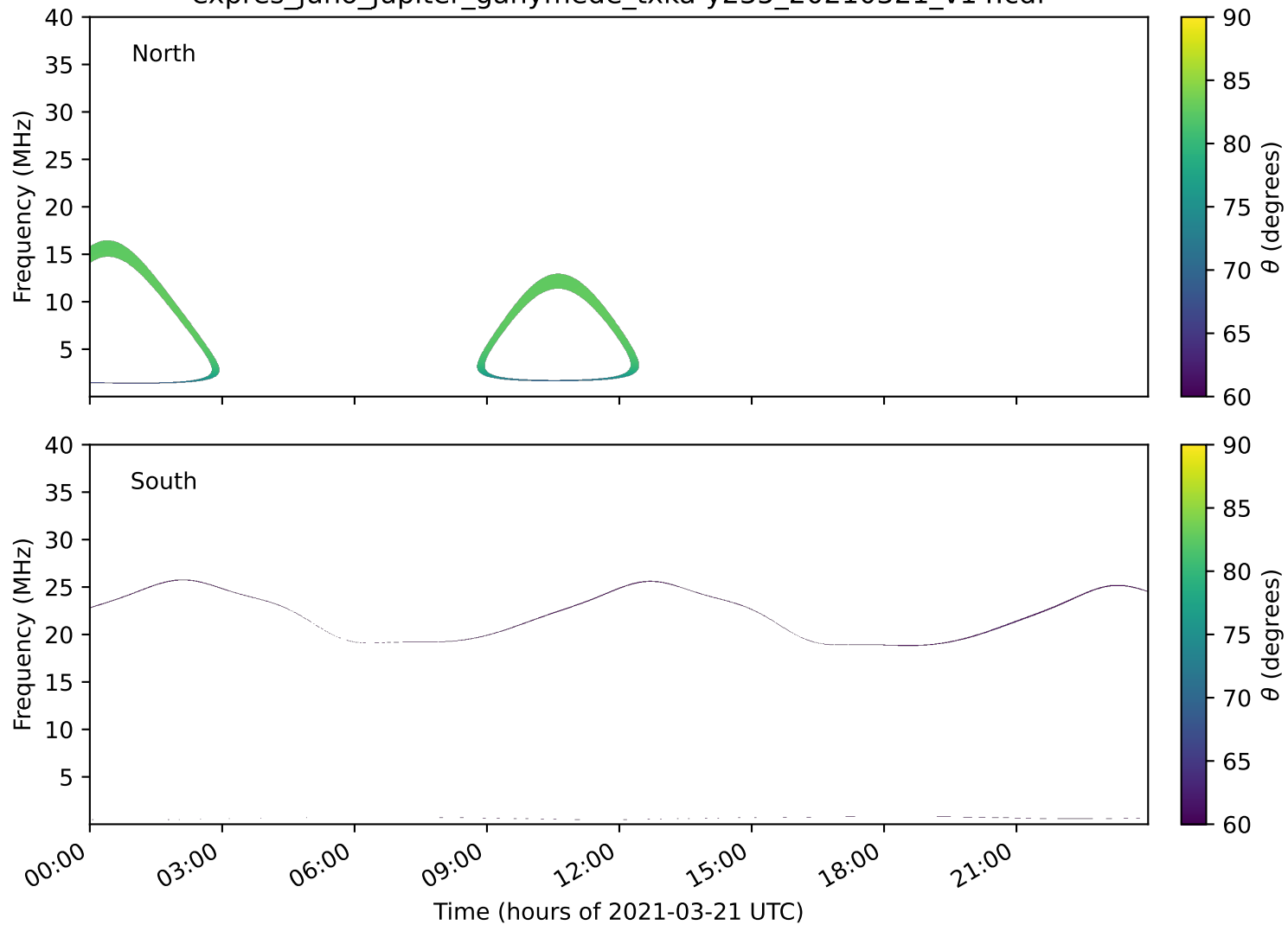
expres_juno_jupiter_ganymede_txka-y235_20210321_v14.cdf
