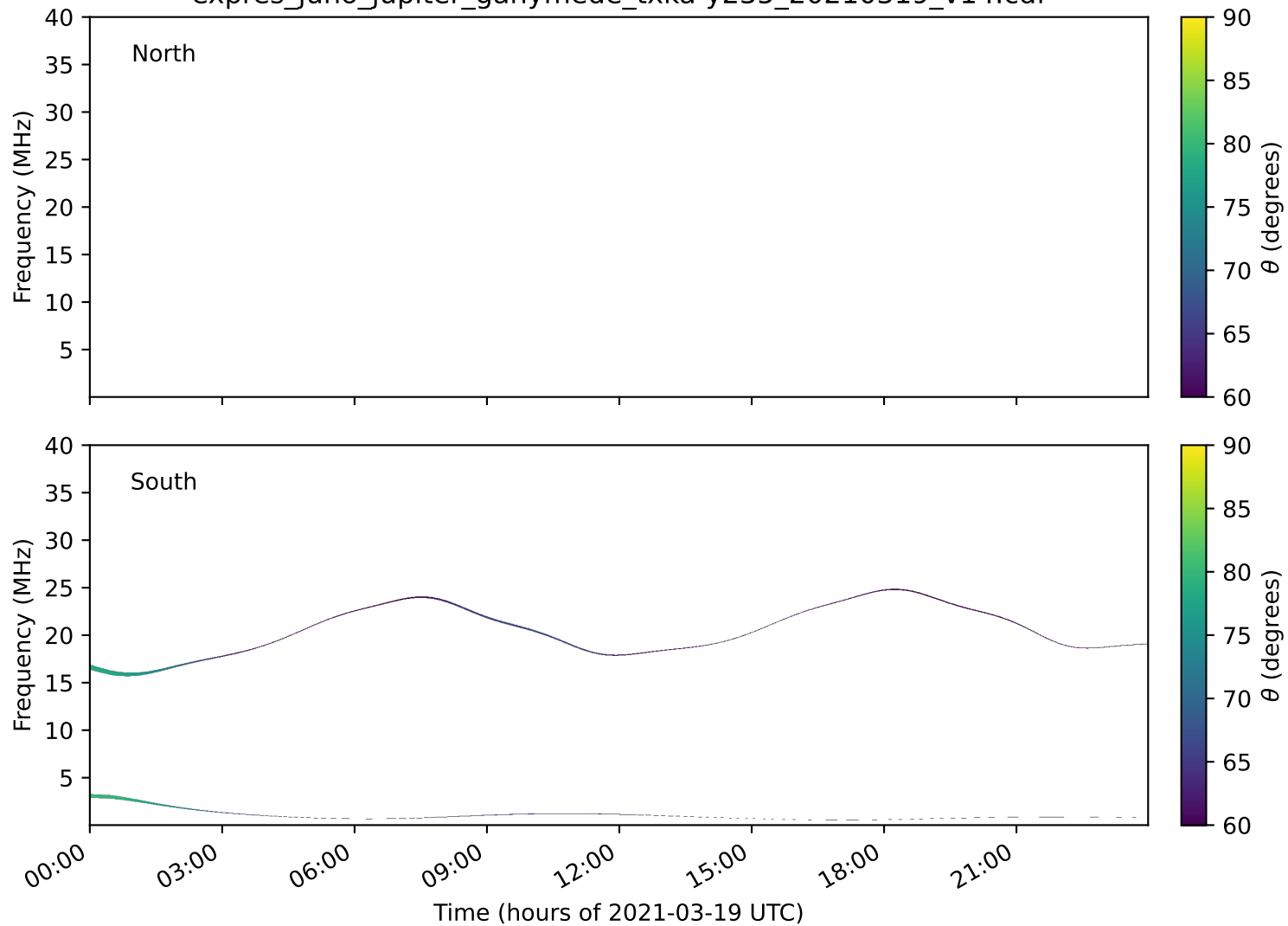
expres_juno_jupiter_ganymede_txka-y235_20210319_v14.cdf
